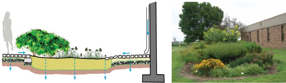
Figure 14. Rain garden
