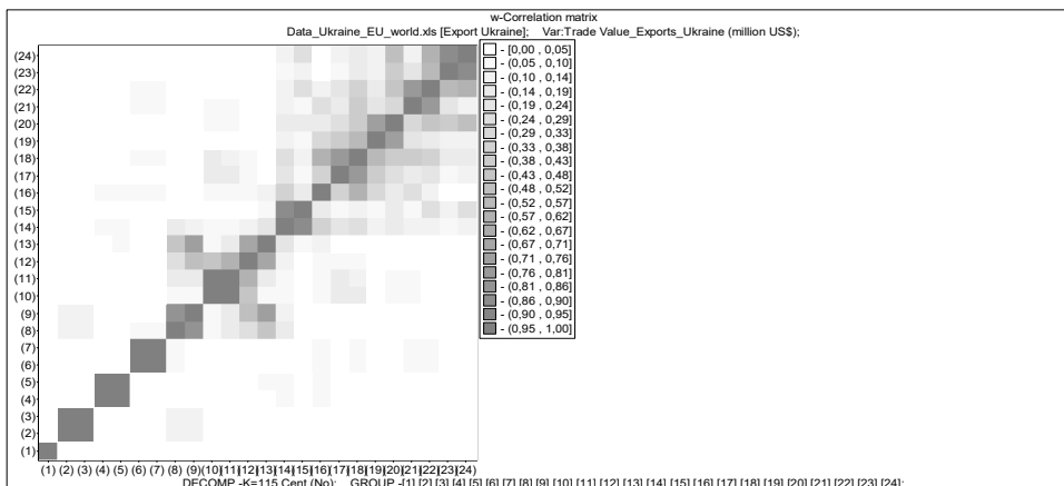
Figure 3. Correlation matrix of multidimensional series of observations
