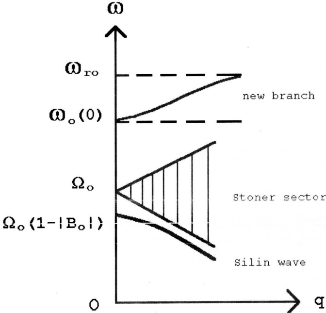
Fig.3. The dispersion curve (3.9) location at n = 0 relatively to the Stoner sector and the Silin wave spectrum.
