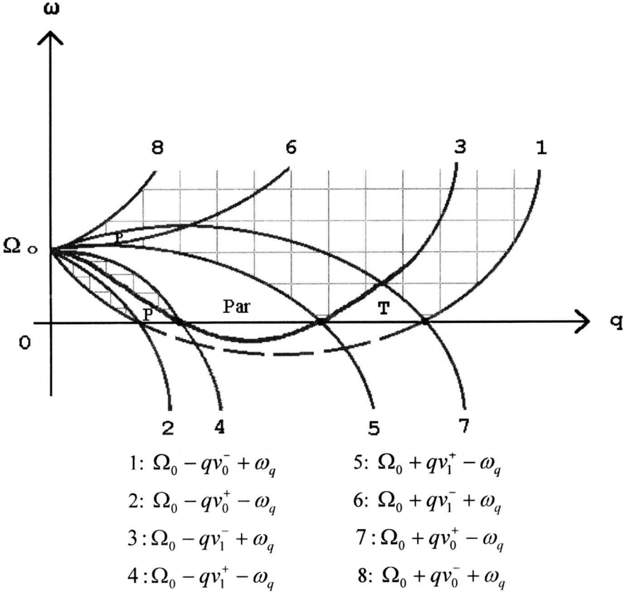
Fig.8. The Landau damping regions and transparency windows for the spin waves in the case of the two filled Landau zones.
