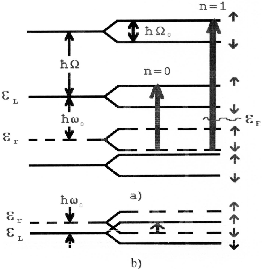
Fig.2. Resonance transitions QL \downarrow \rightarrow LL \uparrow :
