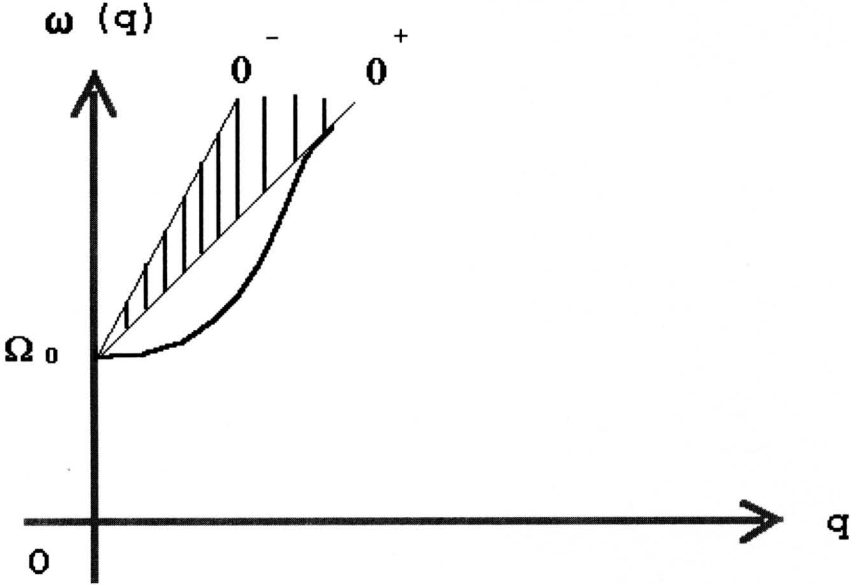
Fig.10. The dispersion curve of the quantum spin waves in the parabolic transparency window without taking into account the quasi-local states at two filled Landau sublevels 0^\pm .
