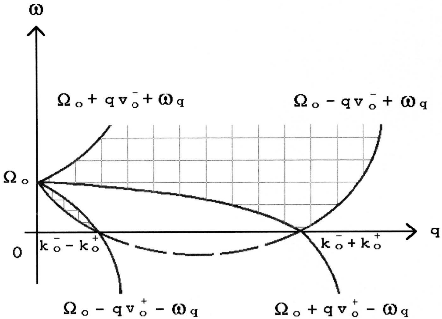
Fig. 7. The regions of collisionless wave damping in the case of one filled Landau zone.
