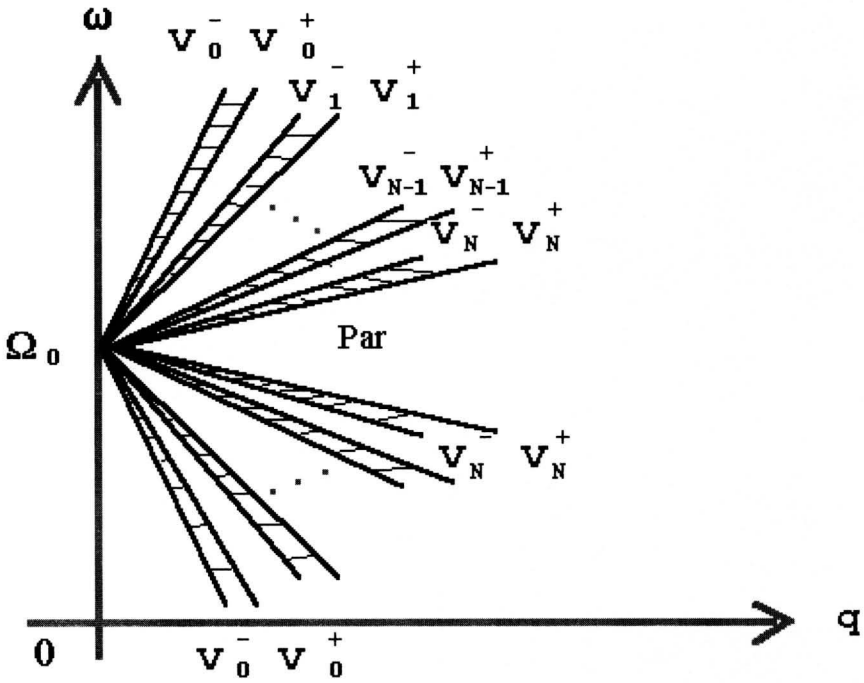
Fig.9. The Landau damping regions in the long-wavelength limit.
