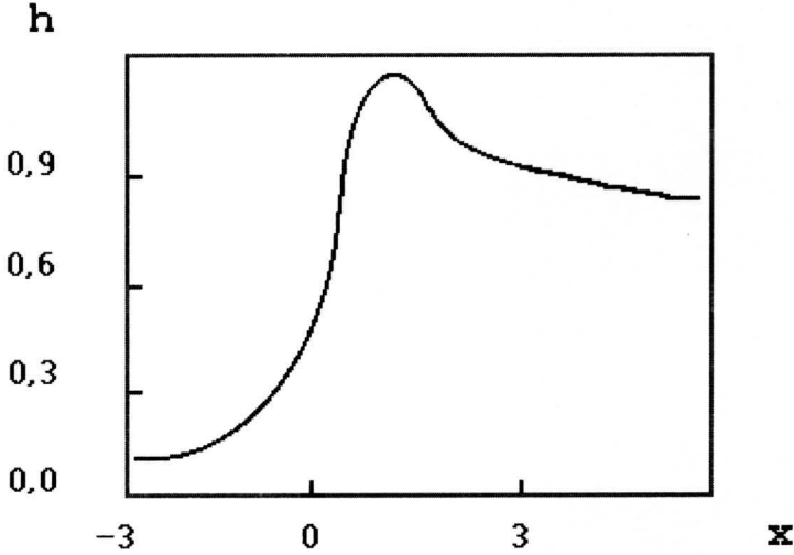
Fig. 12. The dependence of the neutron scattering cross-section on the value of energy loss near the frequency \omega_m .
