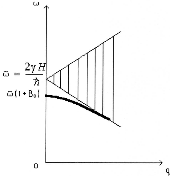
Fig. 1. The dispersion curve (1.11) for the spin waves of Silin ( B_0 < 0 ) [26].
