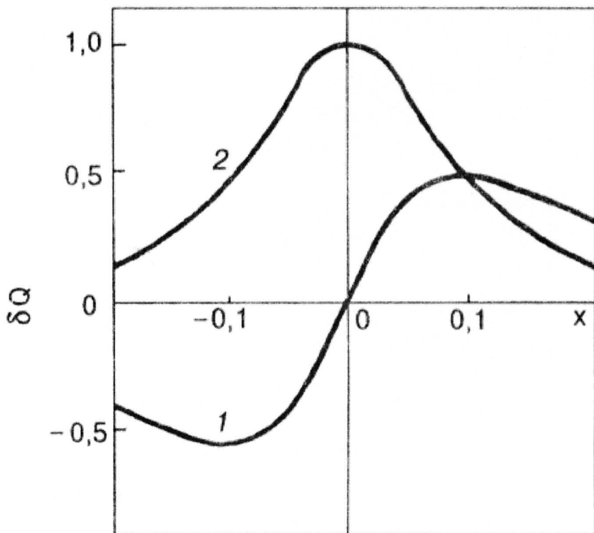
Fig. 13. The dependence of the real (1) and the imaginary (2) parts of susceptibility (5.14) on the frequency in the neighbourhood of the resonance.
