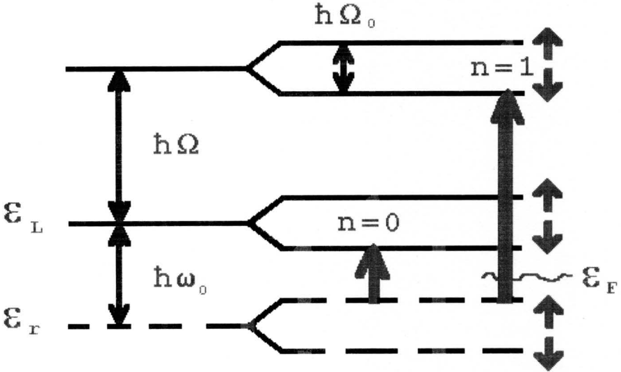
Fig. 6. The resonance transitions QL \uparrow \rightarrow LL \downarrow .
