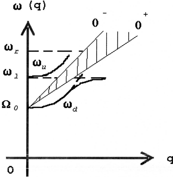
Fig. 11. Two branches of the quantum spin wave spectrum.
