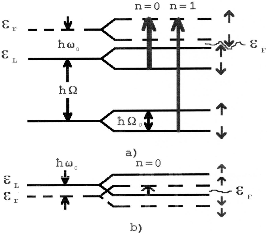
Fig. 4. Resonance transitions LL \downarrow \rightarrow QL \uparrow :
